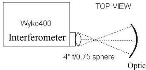
Fig. 11: Azimuthal figure error test geometry.
