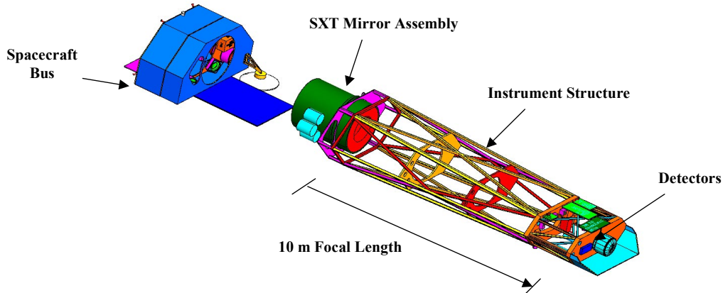
Fig. 1: Constellation-X spacecraft configuration.
