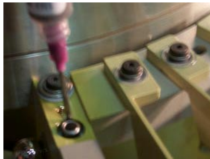
Fig. 14: Example of mounting bushing assembly technique.
