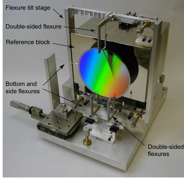
Figure 1. Ultra-low-stress thin-foil optic metrology holder, holding a 100 mm diameter silicon wafer that serves as grating substrate.
