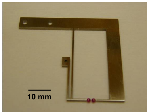
Figure 2. One of three double-sided flexures for the thin foil holder.
