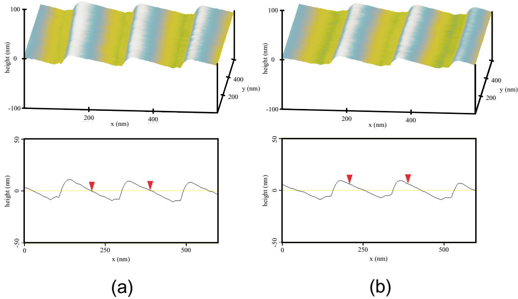
Figure 3. Atomic force micrographs of 200 nm period sawtooth grating replicated via nanoimprint lithography. (a) Thermal-cure NIL. (b) UV-cure NIL.
