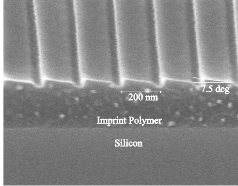
Figure 4. Scanning electron micrograph of a grating replica made by thermal-cure NIL. The groove profile is sharper than in Fig. 3(a) due to the absence of AFM tip size artefacts.
