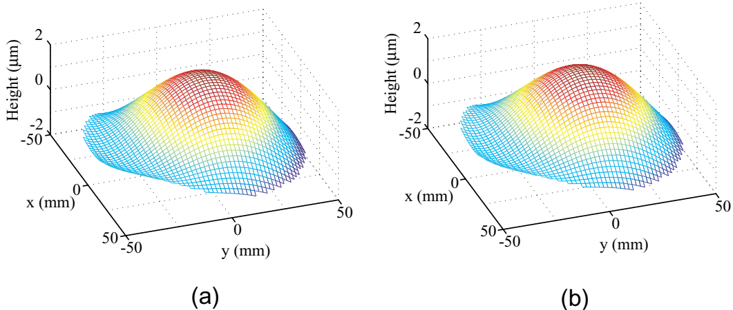
Figure 5. Silicon wafer surface map reconstruction from Shack-Hartmann data. (a) Before NIL ( 3.601 \mu\text{m} P-V). (b) After thermal-cure NIL ( 3.625 \mu\text{m} P-V).
